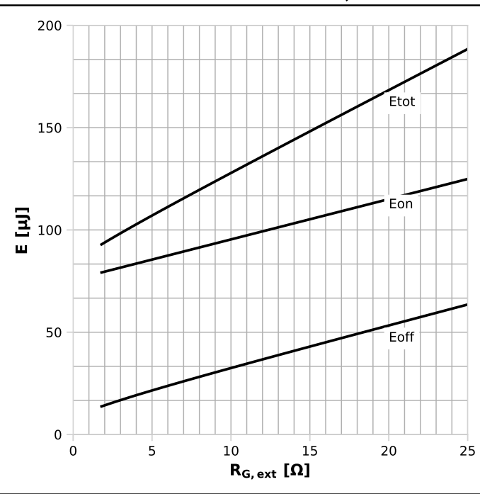
Diagram 18: Typ. Switching Losses vs R_{G,ext}
