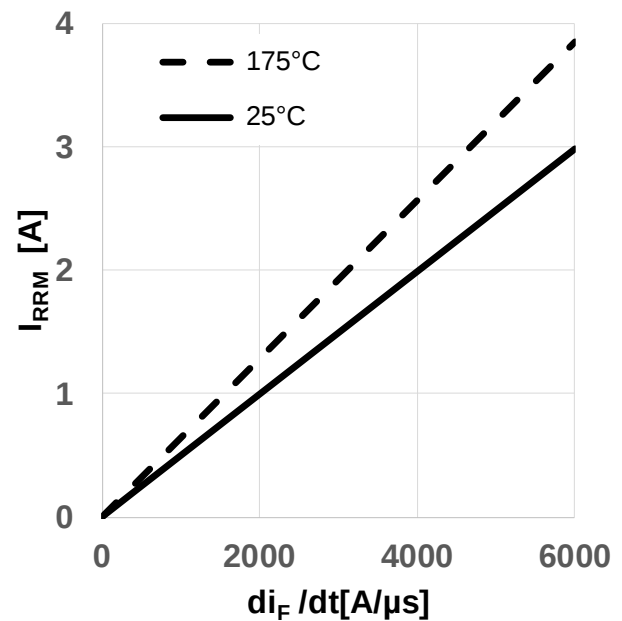
Figure 20 Typical reverse recovery current as a function of diode current slope (I_{rrm} = f(di_F/dt), V_{DD} = 800V, V_{GS} = 0V/18V, I_D = 2A, \text{ind. load, test circuit in Fig. E, body diode at } V_{GS} = 0V)
