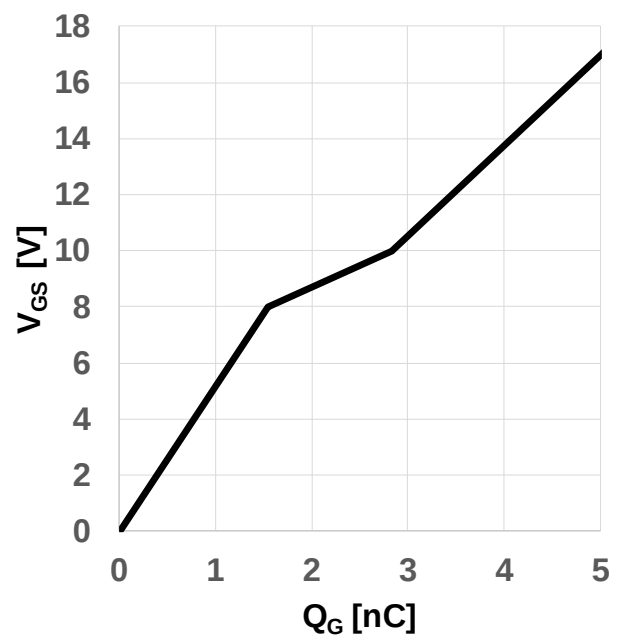
Figure 10 Typical gate charge (V_{GS} = f(Q_G), I_{DS} = 2A, V_{DS} = 800V, \text{turn-on pulse})
