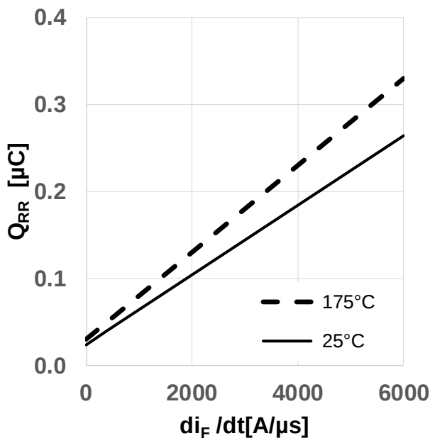
Figure 19 Typical reverse recovery charge as a function of diode current slope (Q_{rr} = f(di_F/dt), V_{DD} = 800V, V_{GS} = 0V/18V, I_D = 2A, \text{ind. load, test circuit in Fig. E, body diode at } V_{GS} = 0V)
