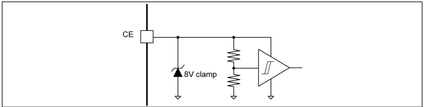
Figure 66 ESD protection and pin diagram for CE pin
