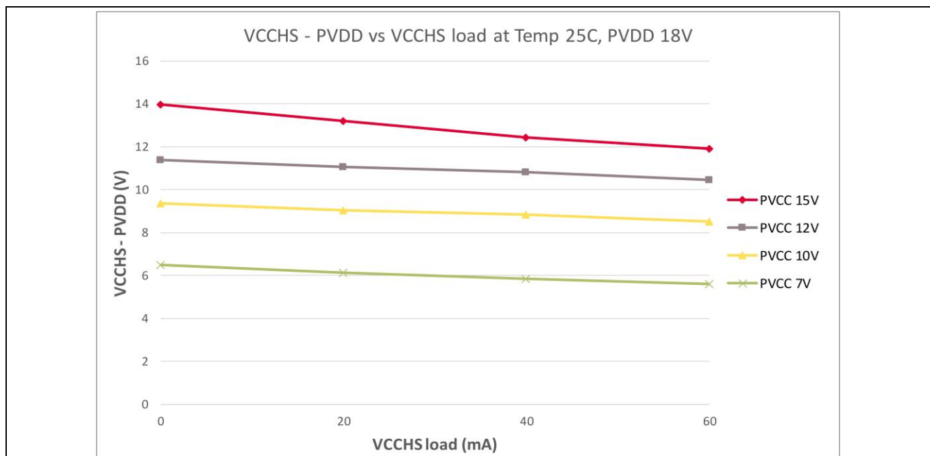
Figure 11 VCCHS average voltage vs VCCHS load (DC) for different PVCC configurations at PVDD 18V. XMC active and executing code. Typical application with C_{CP1(2)} = 220\text{nF} and C_{VCCLS/HS} = 1\mu\text{F} . VCCLS load 20mA.
