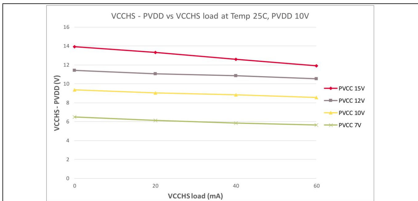
Figure 12 VCCHS average voltage vs VCCHS load (DC) for different PVCC configurations at PVDD 10V. XMC active and executing code. Typical application with C_{CP1(2)} = 220\text{nF} and C_{VCCLS/HS} = 1\mu\text{F} . VCCLS load 20mA
