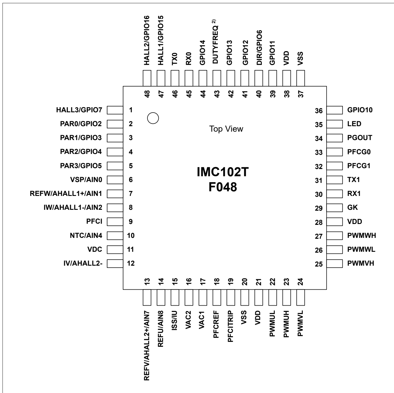
Figure 7 IMC102T-F048
