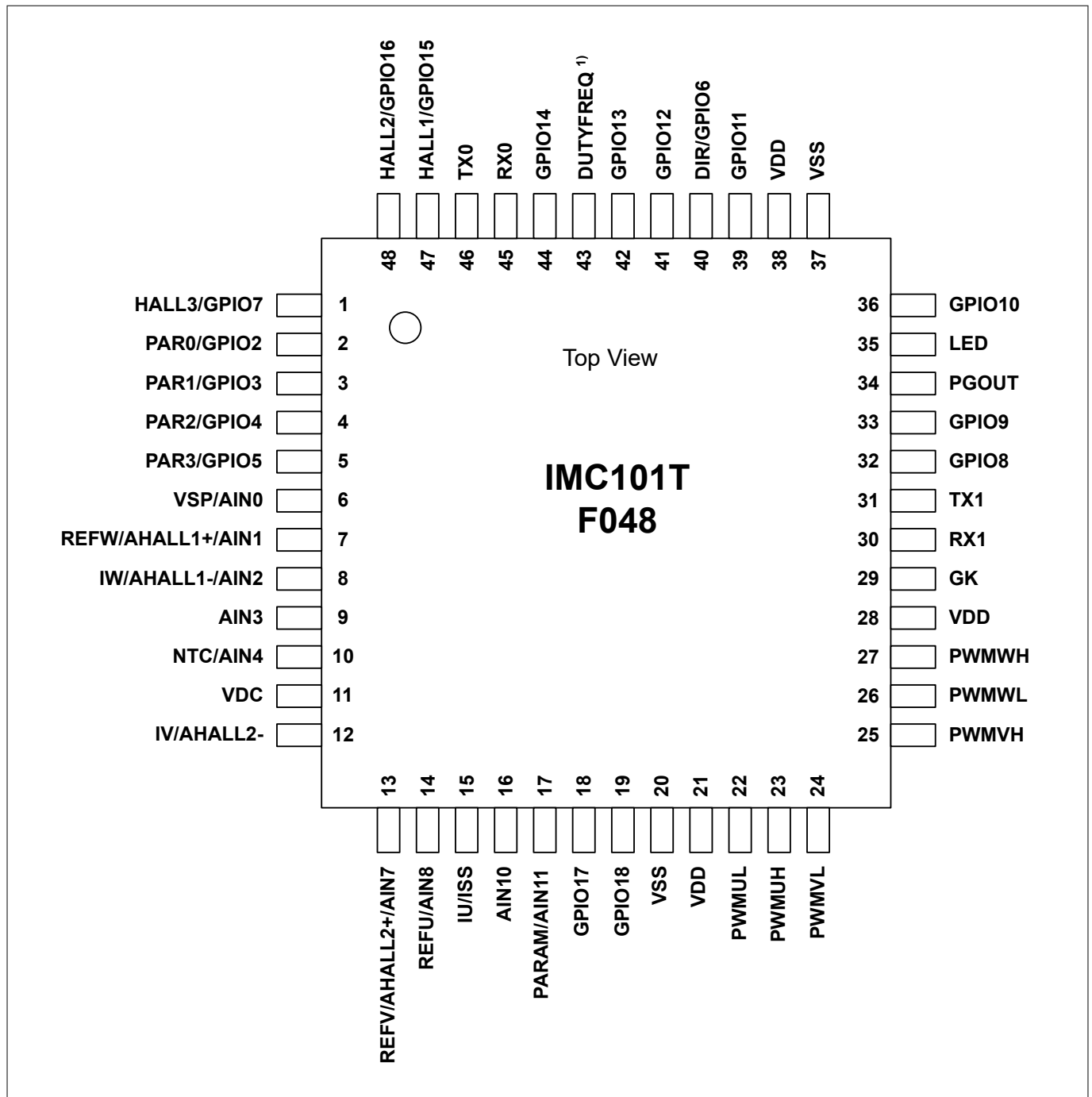
Figure 5 IMC101T-F048
