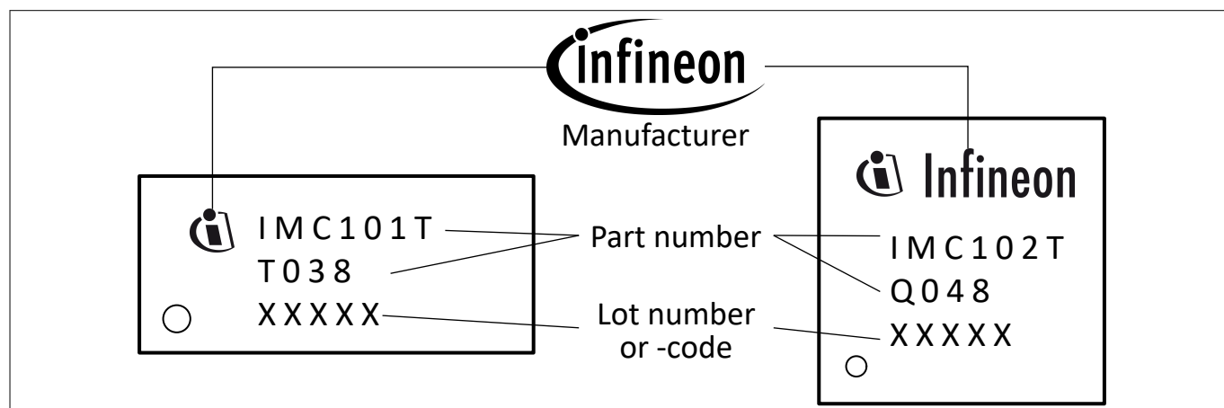
Figure 27 Part marking
