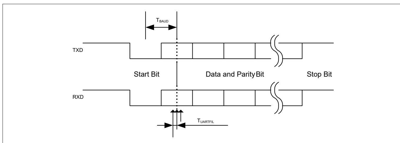
Figure 19 UART timing
