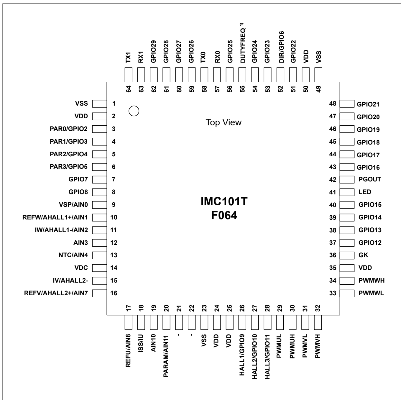
Figure 6 IMC101T-F064
