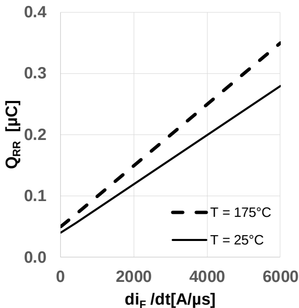
Figure 19 Typical reverse recovery charge as a function of diode current slope (Q_{rr} = f(di_i/dt), V_{DD} = 800V, V_{GS} = 0V/18V, I_D = 4A, \text{ind. load, test circuit in Fig. E, body diode at } V_{GS} = 0V)
