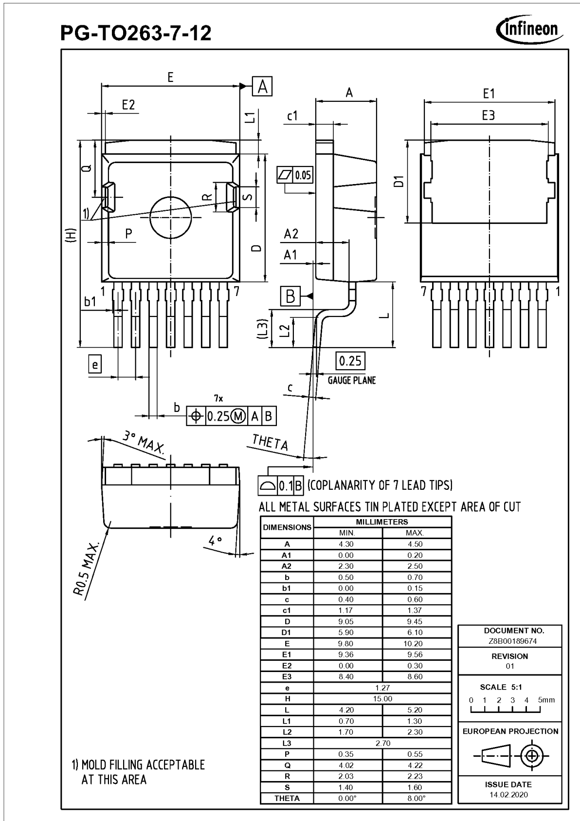
Figure 22 Package drawing
