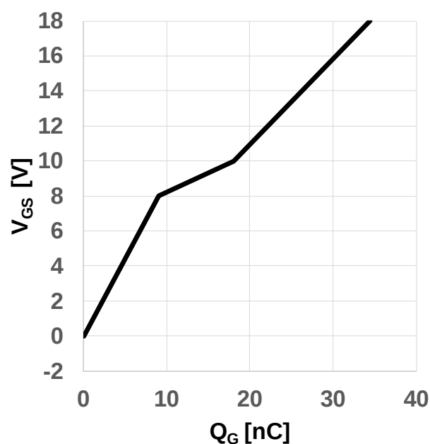
Figure 10 Typical gate charge (V_{GS} = f(Q_G), I_{DS} = 13A, V_{DS} = 800V, \text{turn-on pulse})
