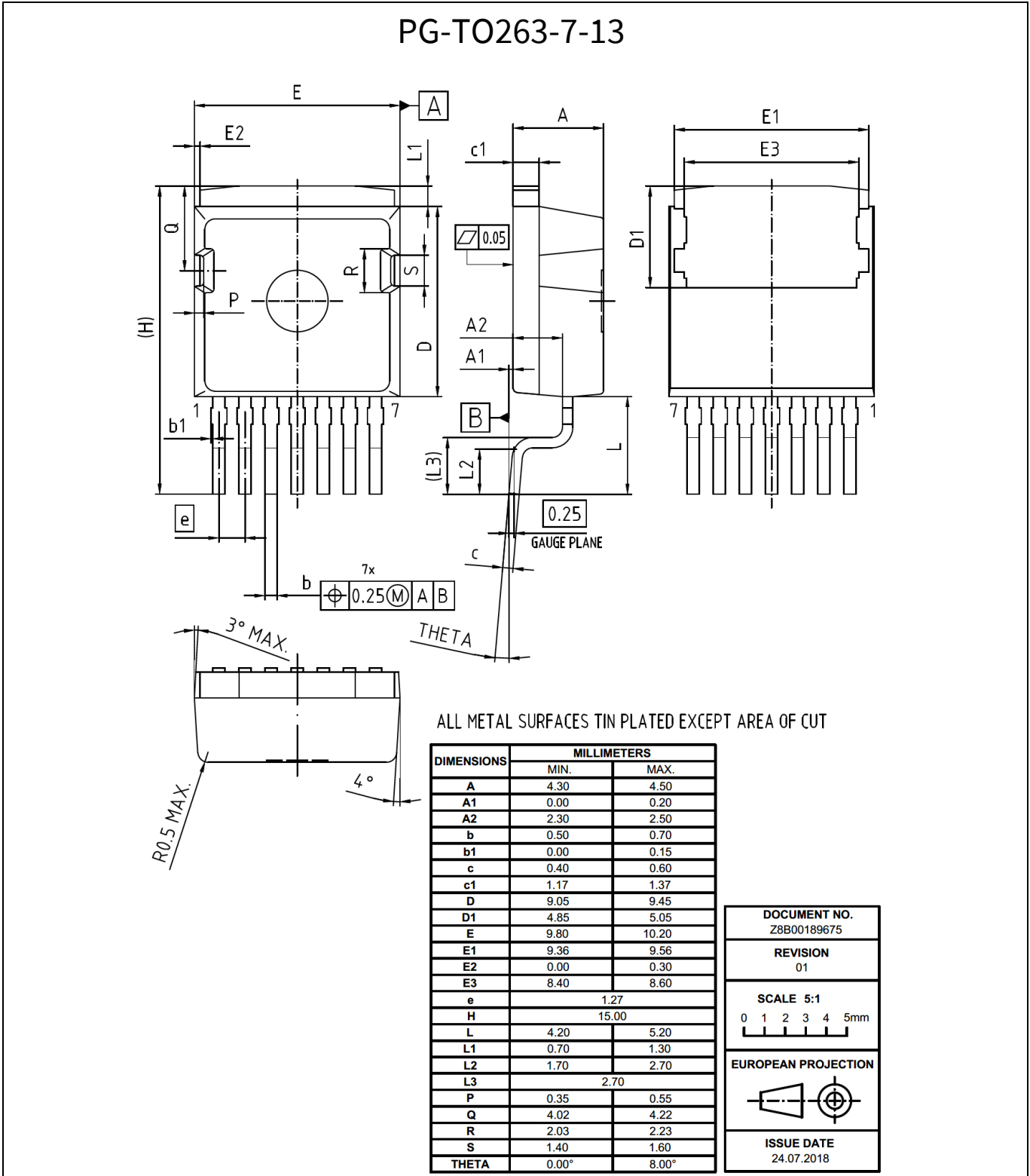
Figure 16 Package drawing
