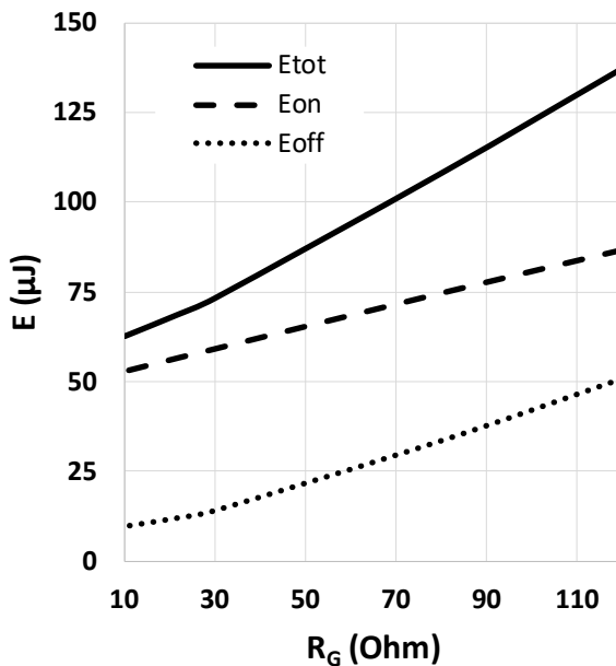
Figure 11 Typical switching energy losses as a function of gate resistance (E = f(R_{G,ext}), V_{DD} = 1000V, V_{GS} = 0V/12V, I_D = 1.5A, T_{vj} = 175^\circ C, \text{ind. load, test circuit in Fig. E, diode: body diode at } V_{GS} = 0V)
