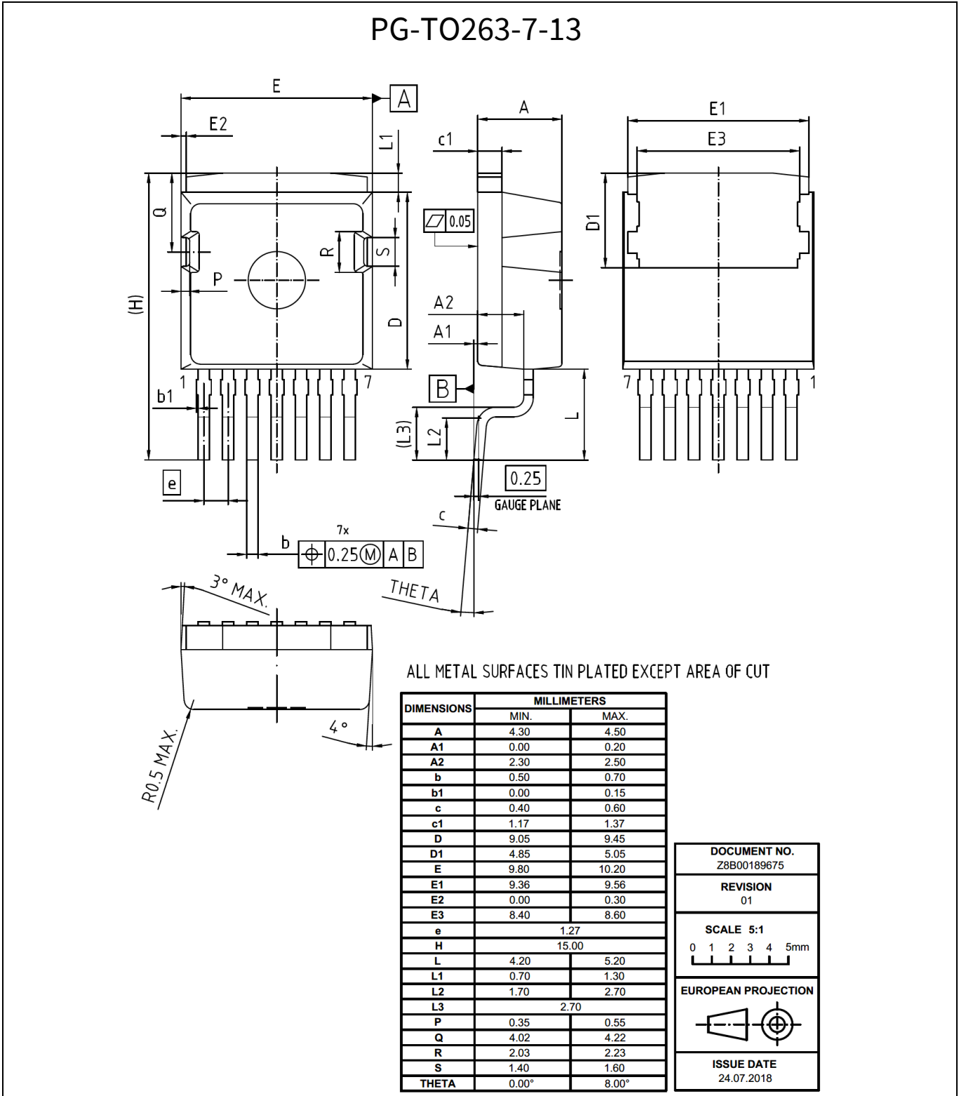
Figure 16 Package drawing
