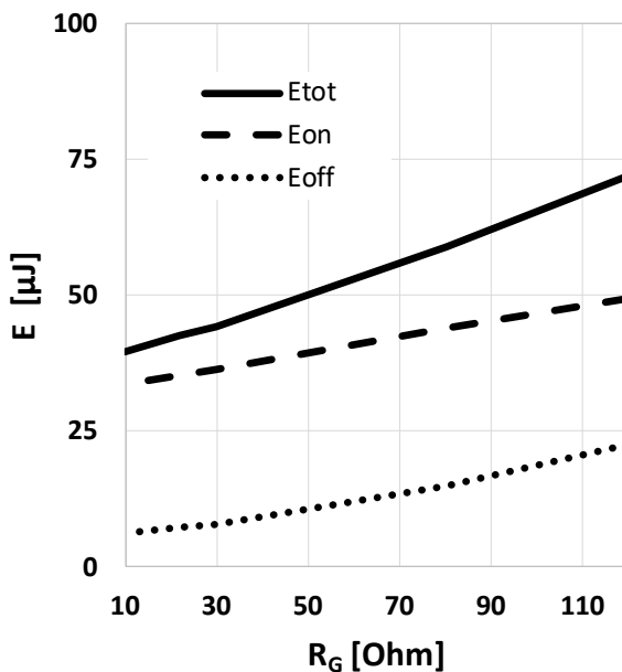
Figure 11 Typical switching energy losses as a function of gate resistance (E = f(R_{G,ext}), V_{DD} = 1000V, V_{GS} = 0V/12V, I_D = 1A, T_{vj} = 175^\circ C, \text{ind. load, test circuit in Fig. E, diode: body diode at } V_{GS} = 0V)
