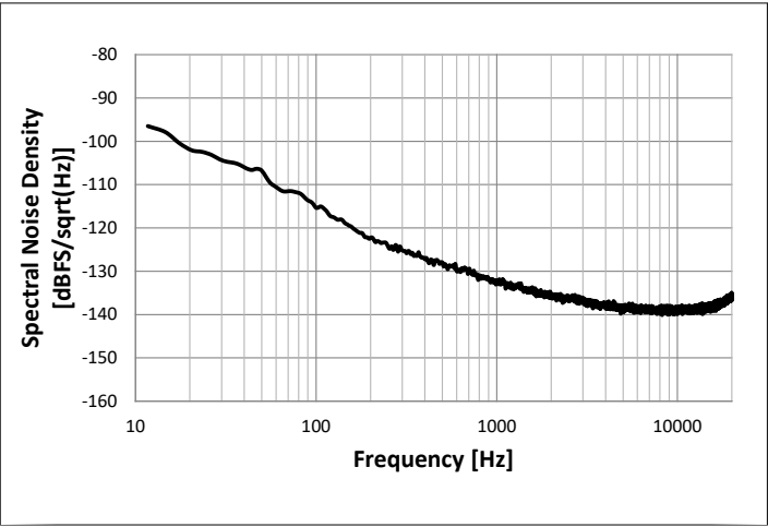
Figure 8 Typical noise floor (unweighted)
