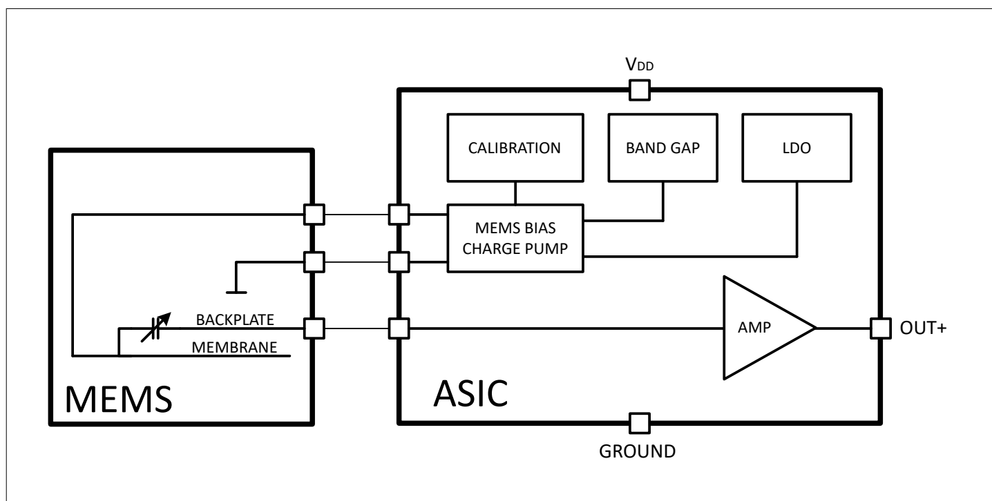
Figure 1 Block diagram
