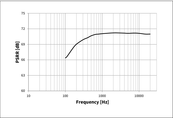
Figure 9 Typical PSRR
