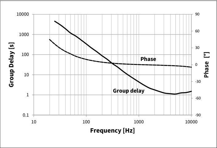
Figure 5 Typical group delay and phase response
