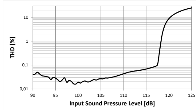
Plot 2: Typical THD vs. SPL
