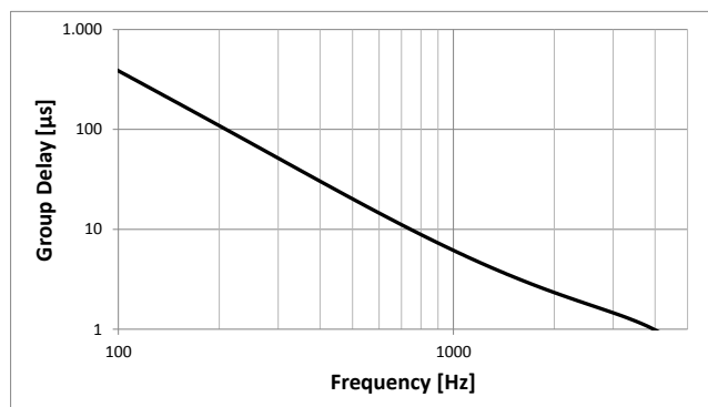
Plot 4: Typical group delay vs. frequency
