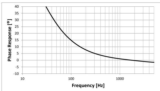
Plot 3: Typical phase response vs. frequency
