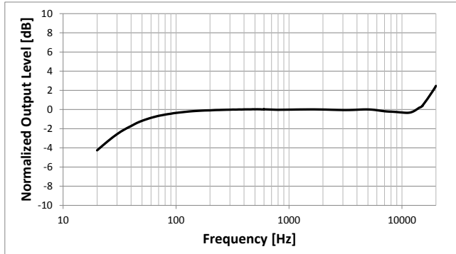
Plot 1: Typical free field response
