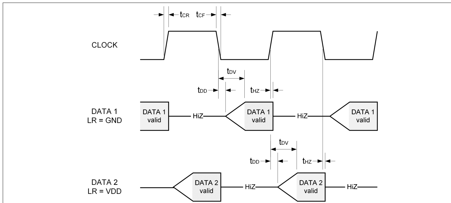
Figure 3 Timing diagram
