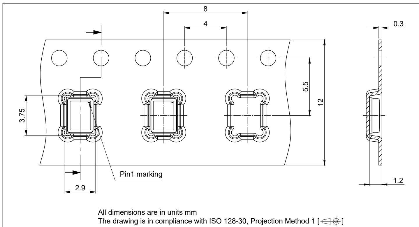
Figure 10 Tape dimensions
