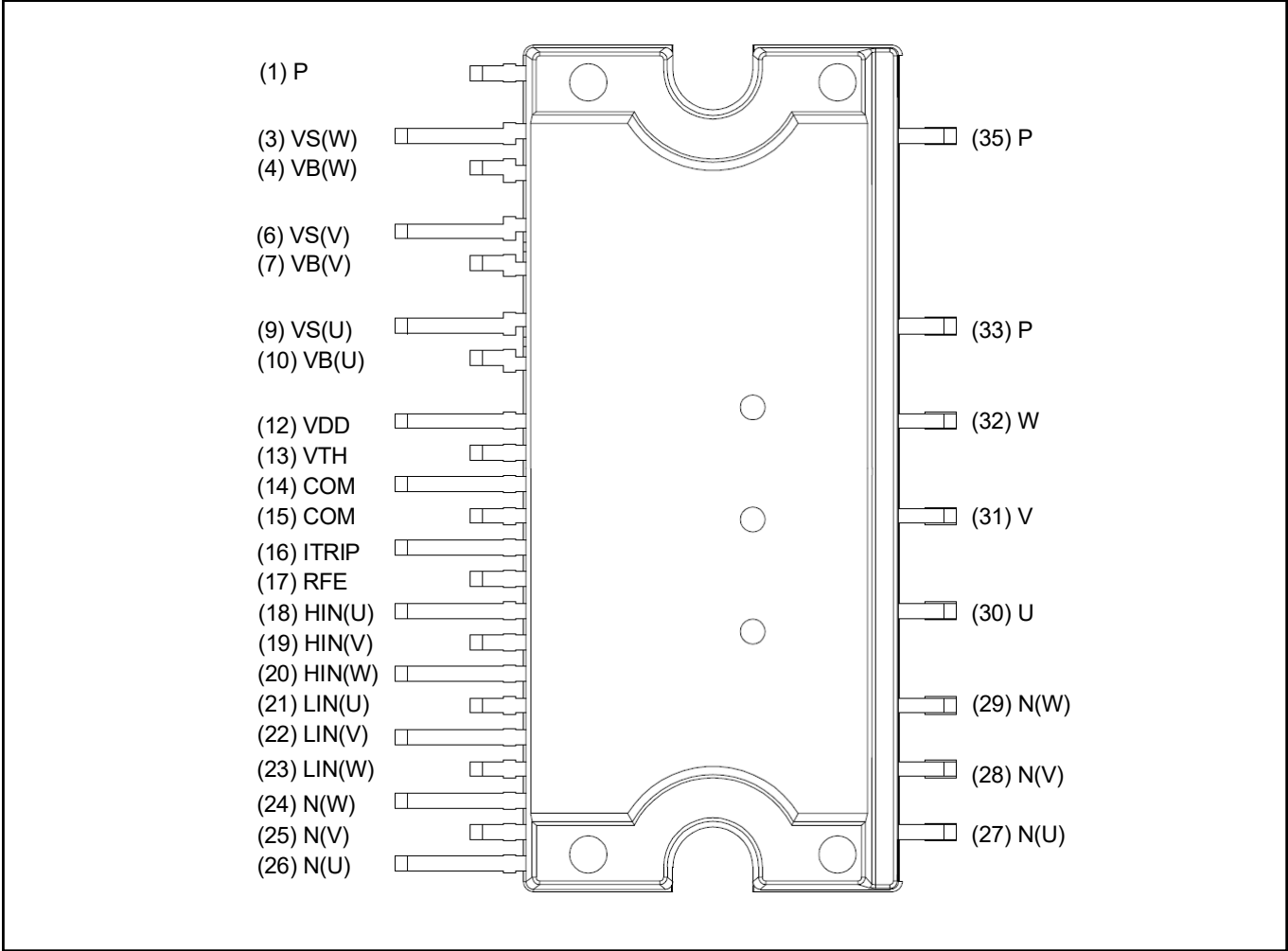
Figure 2 Pin configuration
