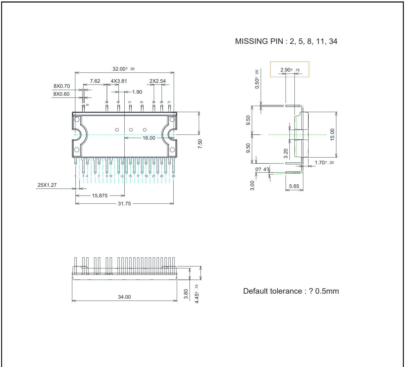
Figure 19 IM393-S6E2
