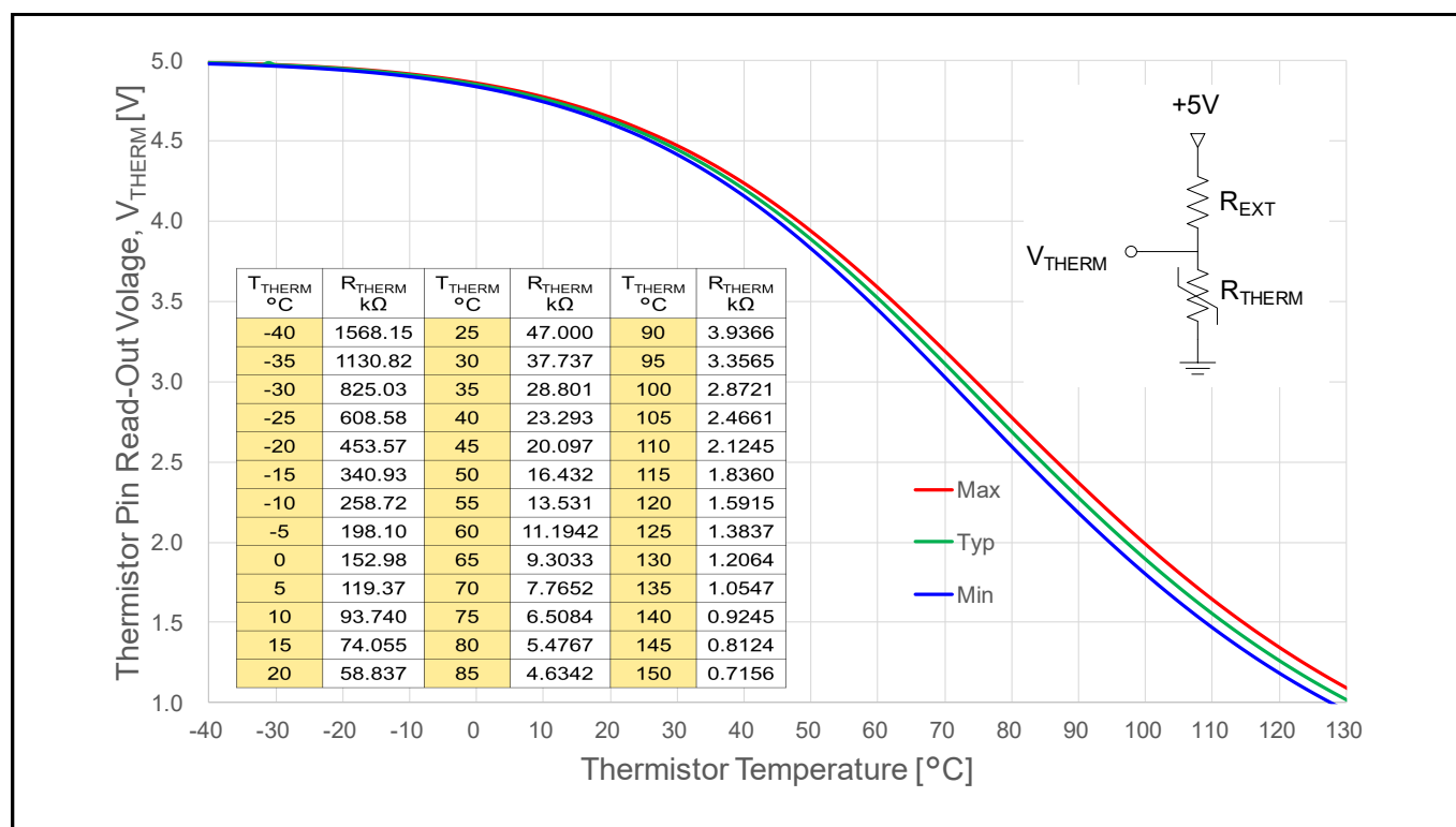
Figure 7 Thermistor readout vs. temperature (with 4.7k \Omega R_{\text{EXT}} pull-up resistor) and typical thermistor resistance values vs. temperature table (For more details, please refer to the application note 'AN2018-13 CIPOS™ IM393-XX IPM technical description_1R0_final')
