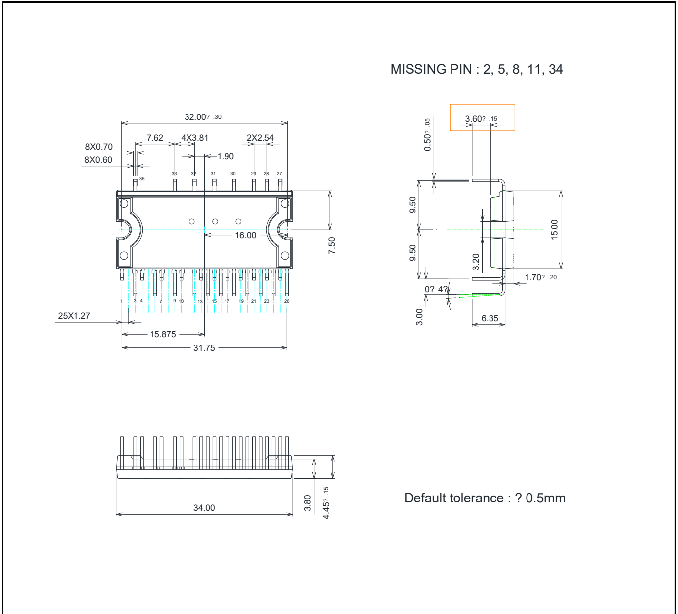
Figure 20 IM393-S6E3
