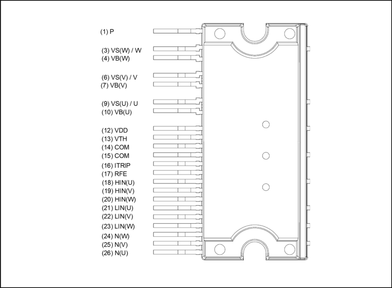
Figure 2 Pin configuration
