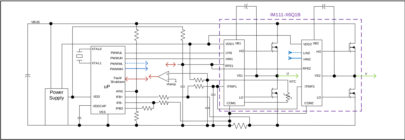
Figure 8 Application schematic
