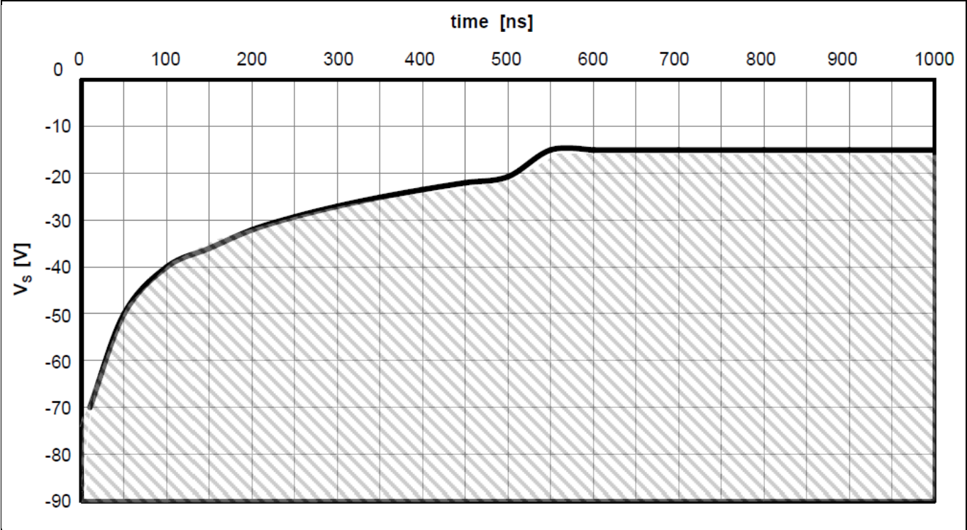
Figure 10 -Vs immunity
