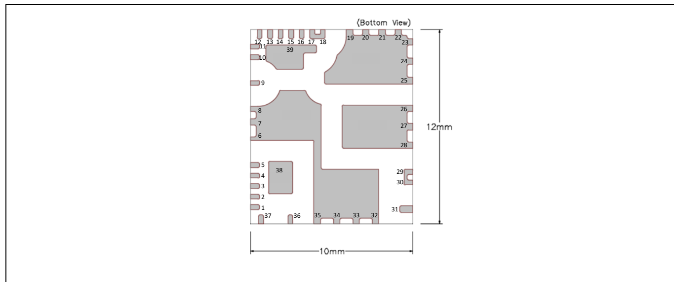
Figure 2 Module pinout
