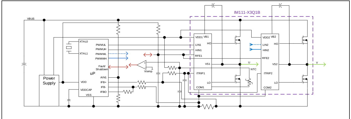
Figure 8 Application schematic
