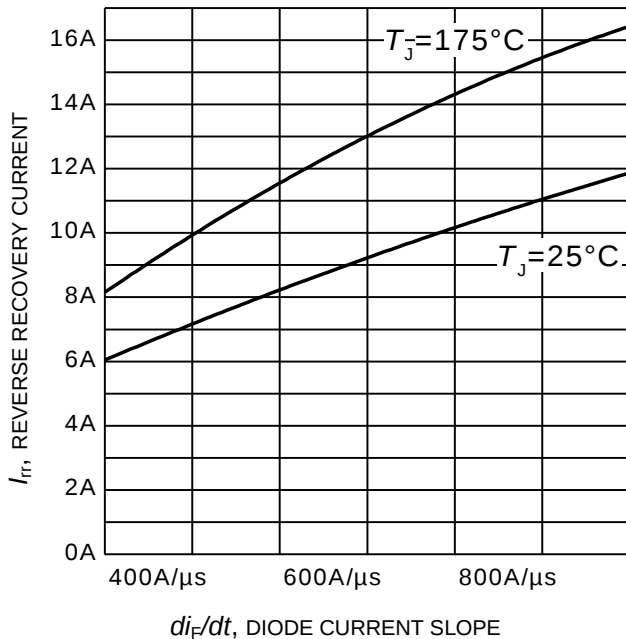
Figure 25. Typical reverse recovery current as a function of diode current slope ( V_R = 400V , I_F = 15A , Dynamic test circuit in Figure E)
