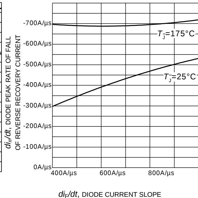
Figure 26. Typical diode peak rate of fall of reverse recovery current as a function of diode current slope ( V_R = 400V , I_F = 15A , Dynamic test circuit in Figure E)
