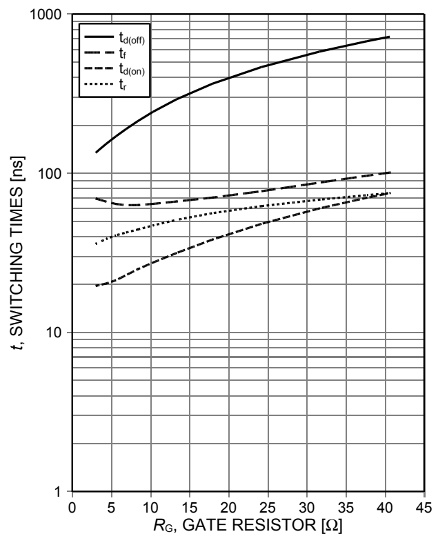
Figure 8. Typical switching times as a function of gate resistor (ind. load, T_j=150^\circ C , V_{CE}=400V , V_{GE}=0/15V , I_C=75A , test circuit in Fig. E)
