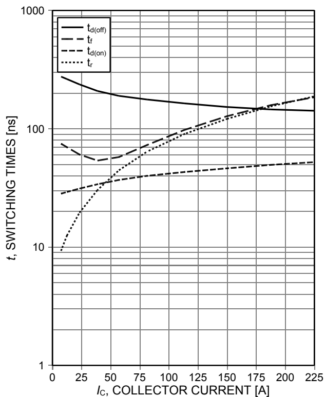
Figure 7. Typical switching times as a function of collector current (ind. load, T_j=150^\circ C , V_{CE}=400V , V_{GE}=0/15V , R_{G(on)}=16\Omega , R_{G(off)}=6\Omega , test circuit in Fig. E)
