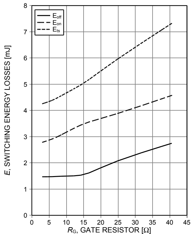
Figure 12. Typical switching energy losses as a function of gate resistor (ind. load, T_j=150^\circ C , V_{CE}=400V , V_{GE}=0/15V , I_C=75A , test circuit in Fig. E)
