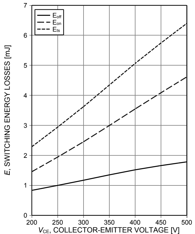
Figure 14. Typical switching energy losses as a function of collector emitter voltage (ind. load, T_J=150^\circ C , V_{GE}=0/15V , I_C=75A , R_{G(on)}=16\Omega , R_{G(off)}=6\Omega , test circuit in Fig. E)
