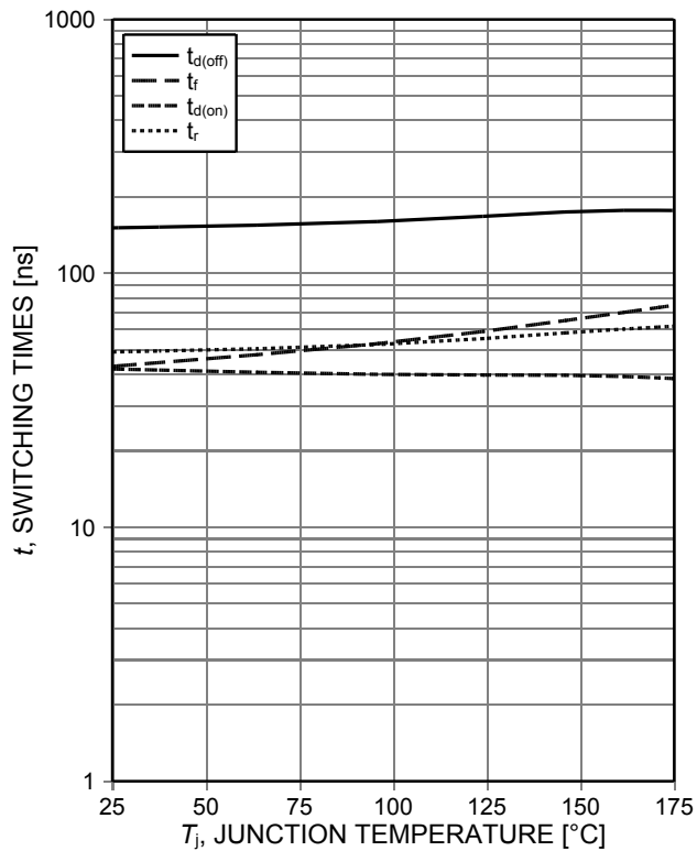
Figure 9. Typical switching times as a function of junction temperature (ind. load, V_{CE}=400V , V_{GE}=0/15V , I_C=75A , R_{G(on)}=16\Omega , R_{G(off)}=6\Omega , test circuit in Fig. E)
