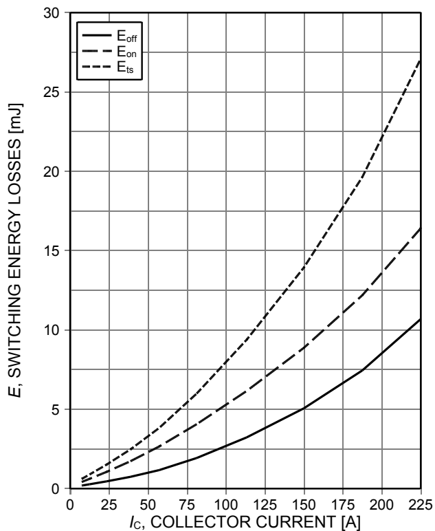
Figure 11. Typical switching energy losses as a function of collector current (ind. load, T_j=150^\circ C , V_{CE}=400V , V_{GE}=0/15V , R_{G(on)}=16\Omega , R_{G(off)}=6\Omega , test circuit in Fig. E)
