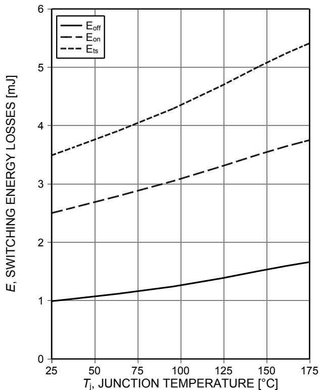
Figure 13. Typical switching energy losses as a function of junction temperature (ind. load, V_{CE}=400V , V_{GE}=0/15V , I_C=75A , R_{G(on)}=16\Omega , R_{G(off)}=6\Omega , test circuit in Fig. E)
