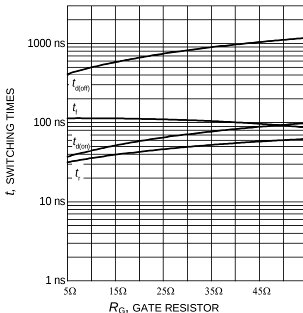
Figure 10. Typical switching times as a function of gate resistor (inductive load, T_J=150^{\circ}\text{C} , V_{CE}=600\text{V} , V_{GE}=0/15\text{V} , I_C=40\text{A} , Dynamic test circuit in Figure E)
