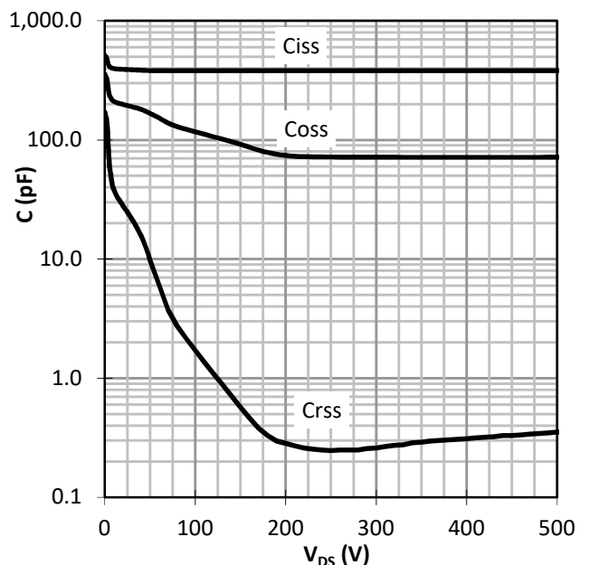
Figure 20 Typ. capacitances
