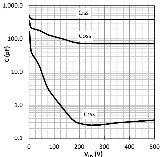
Figure 20 Typ. capacitances
