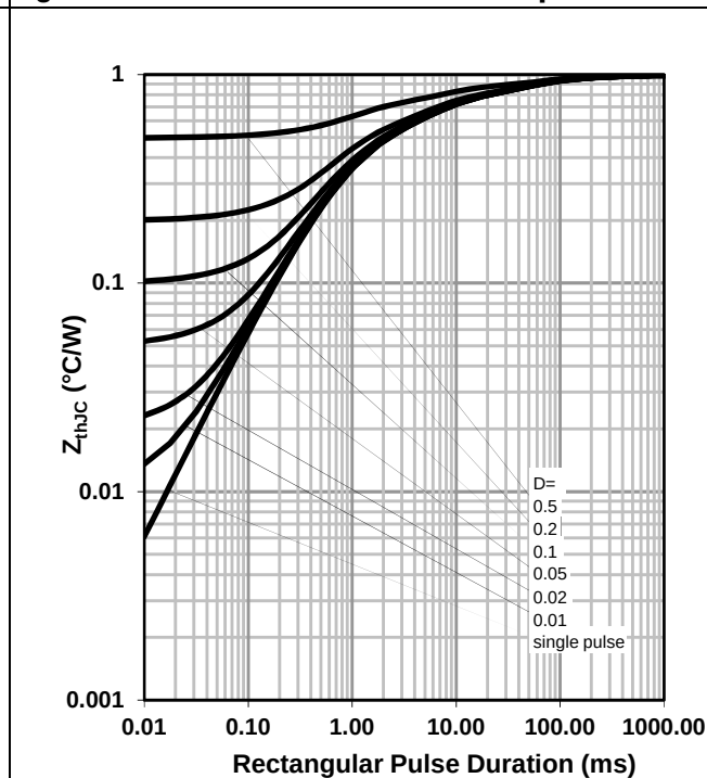
Figure 2 Max. transient thermal impedance
