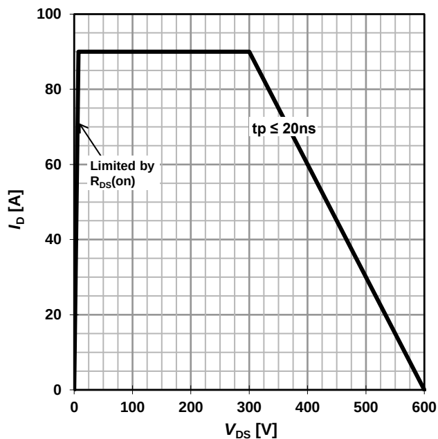
Figure 5 Repetitive safe operating area 1
