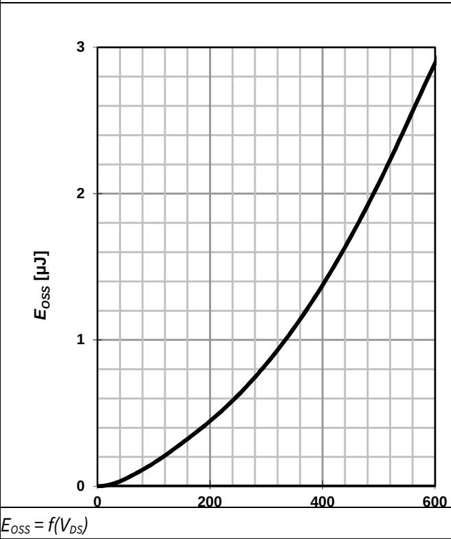
Figure 22 Typ. Coss stored Energy
