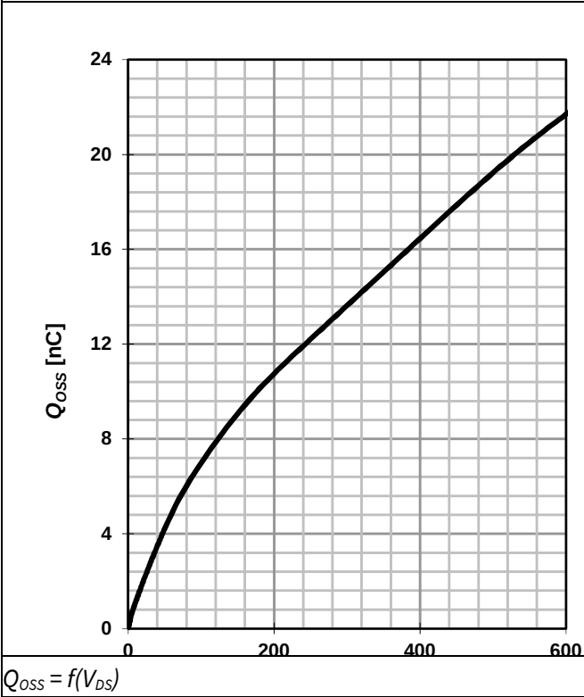
Figure 21 Typ. output charge
