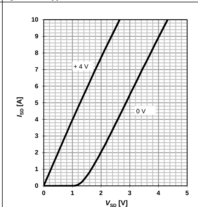
Figure 18 Typ. channel reverse characteristics
