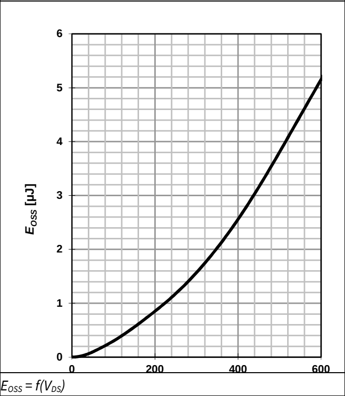
Figure 22 Typ. Coss stored Energy
