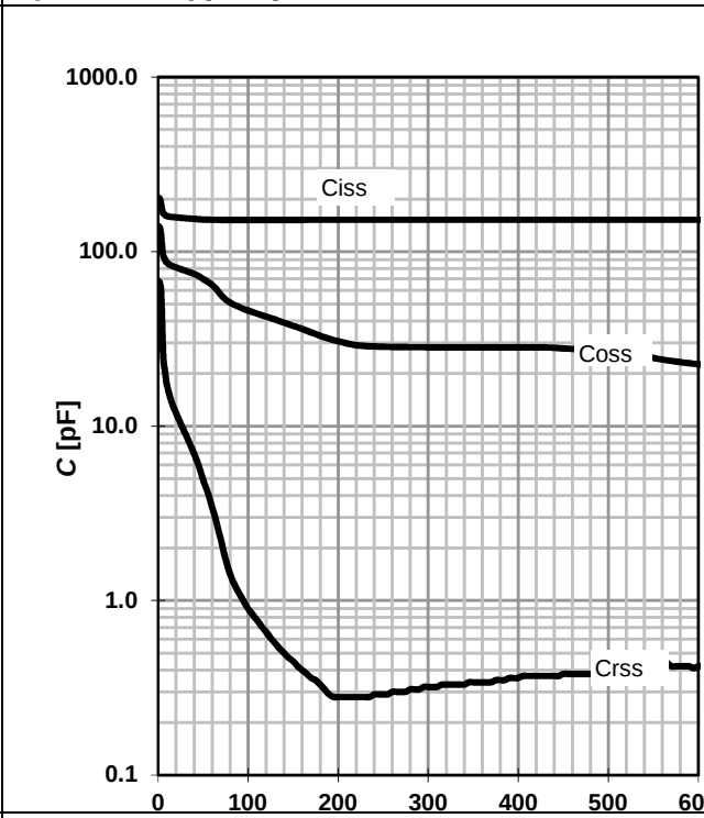
Figure 20 Typ. capacitances
