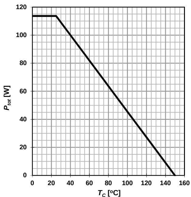
Figure 1 Power dissipation
