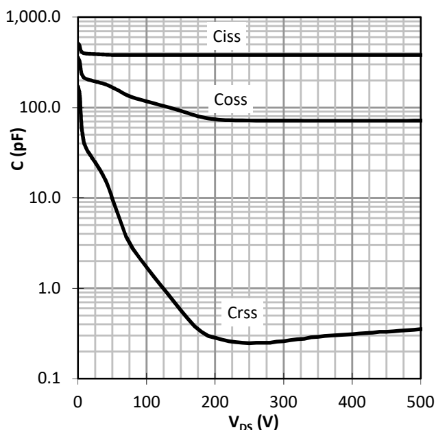
Figure 20 Typ. capacitances
