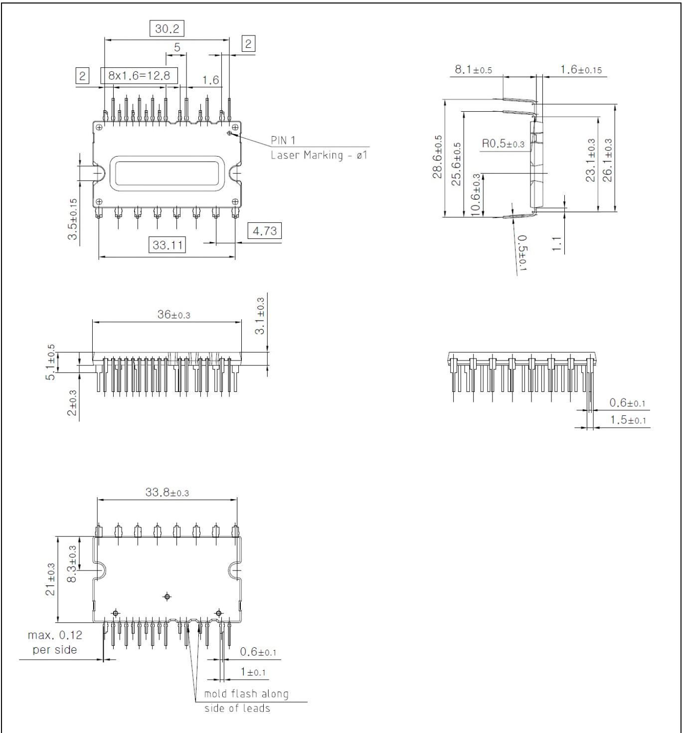
Figure 12 IGCM20F60GA
