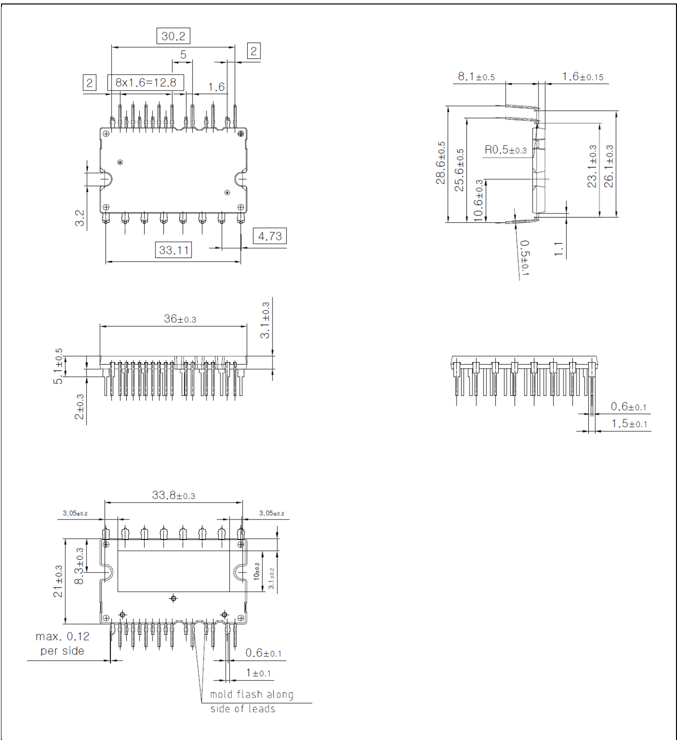
Figure 13 IFCM15S60GD
