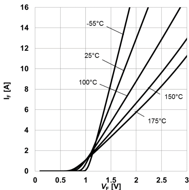
Figure 3. Typical forward characteristics, I_F=f(V_F) , t_p=10\mu\text{s} , parameter: T_{vj}
