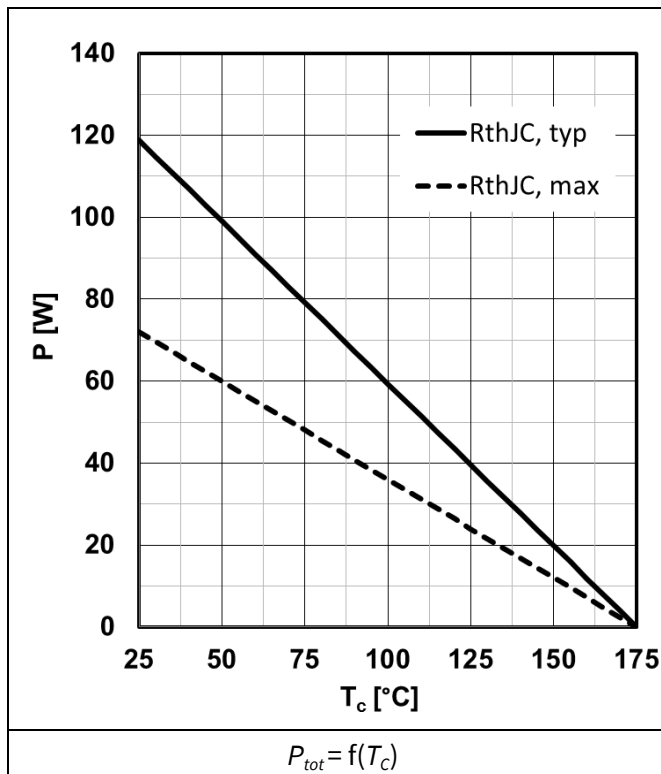
Figure 1 Power dissipation
