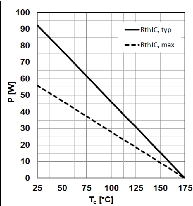
Figure 1 Power dissipation
