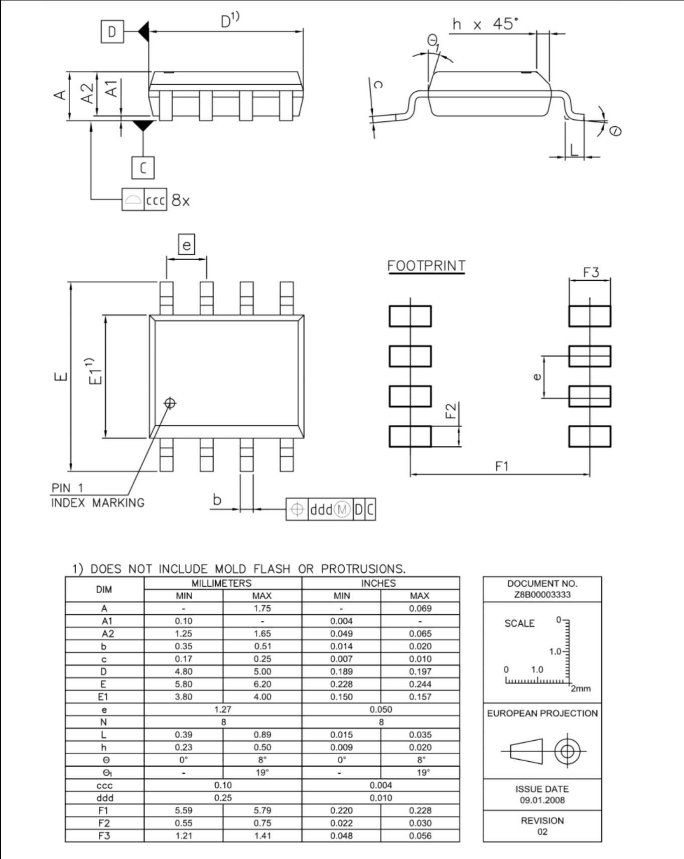
Figure 18 PG-DSO-8
