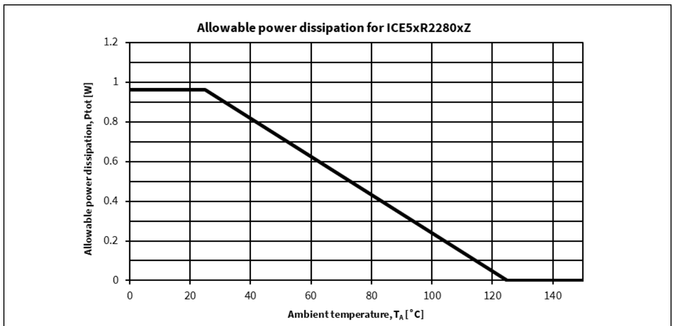
Figure 23 Power dissipation of ICE5xR2280xZ; P_{\text{tot}} = f(T_a) (Maximum ratings as given in chapter 4.1 must not be exceeded)
