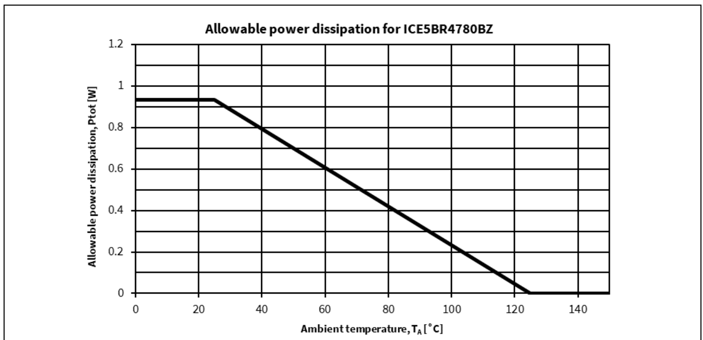
Figure 21 Power dissipation of ICE5BR4780BZ; P_{\text{tot}} = f(T_a) (Maximum ratings as given in chapter 4.1 must not be exceeded)
