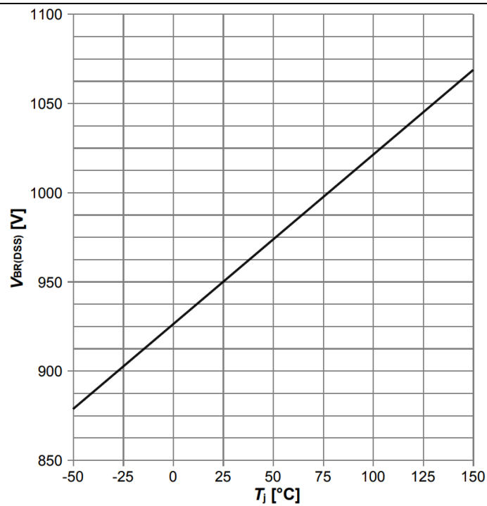
Figure 25 Drain-source breakdown voltage ICE5xR3995xZ; V_{BR(DSS)} = f(T_J) , I_D = 1 mA
