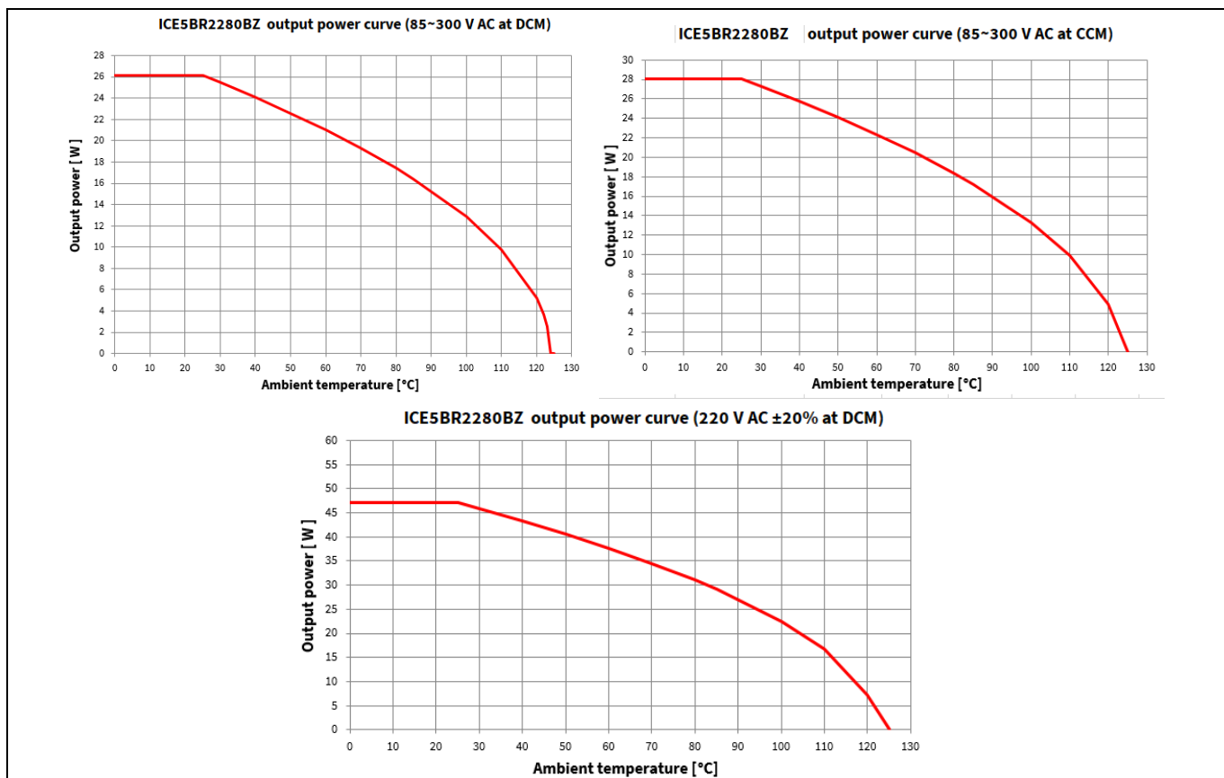
Figure 33 Output power curve of ICE5BR2280BZ
