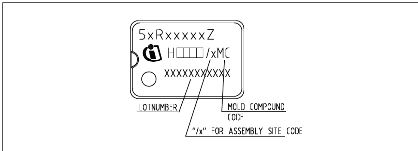
Figure 36 Marking of PG-DIP-7
