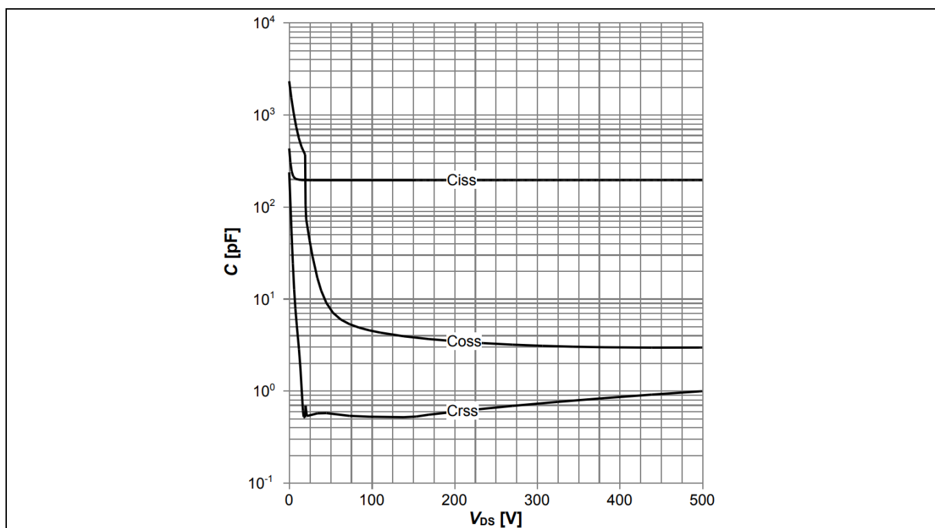
Figure 28 Typical CoolMOS™ capacitances of ICE5xR3995xZ ( C = f(V_{DS}) ; V_{GS} = 0 V; f = 250 kHz)
