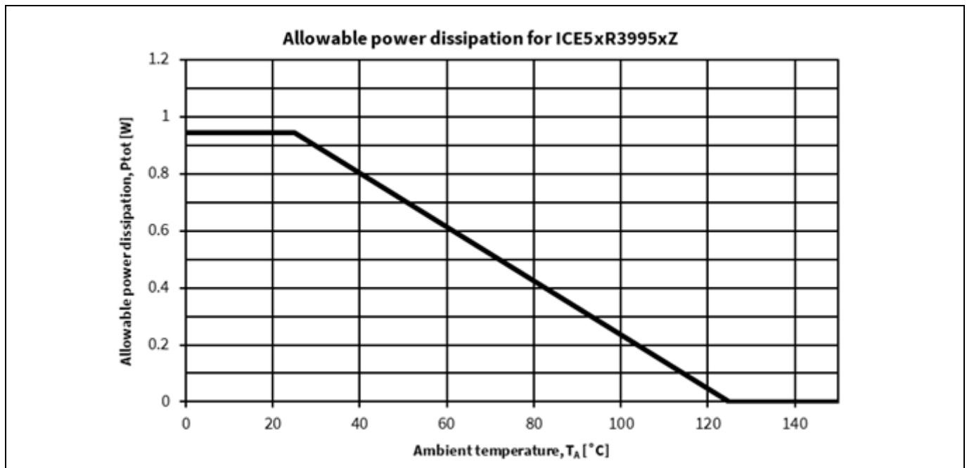
Figure 22 Power dissipation of ICE5xR3995xZ; P_{\text{tot}} = f(T_a) (Maximum ratings as given in chapter 4.1 must not be exceeded)
