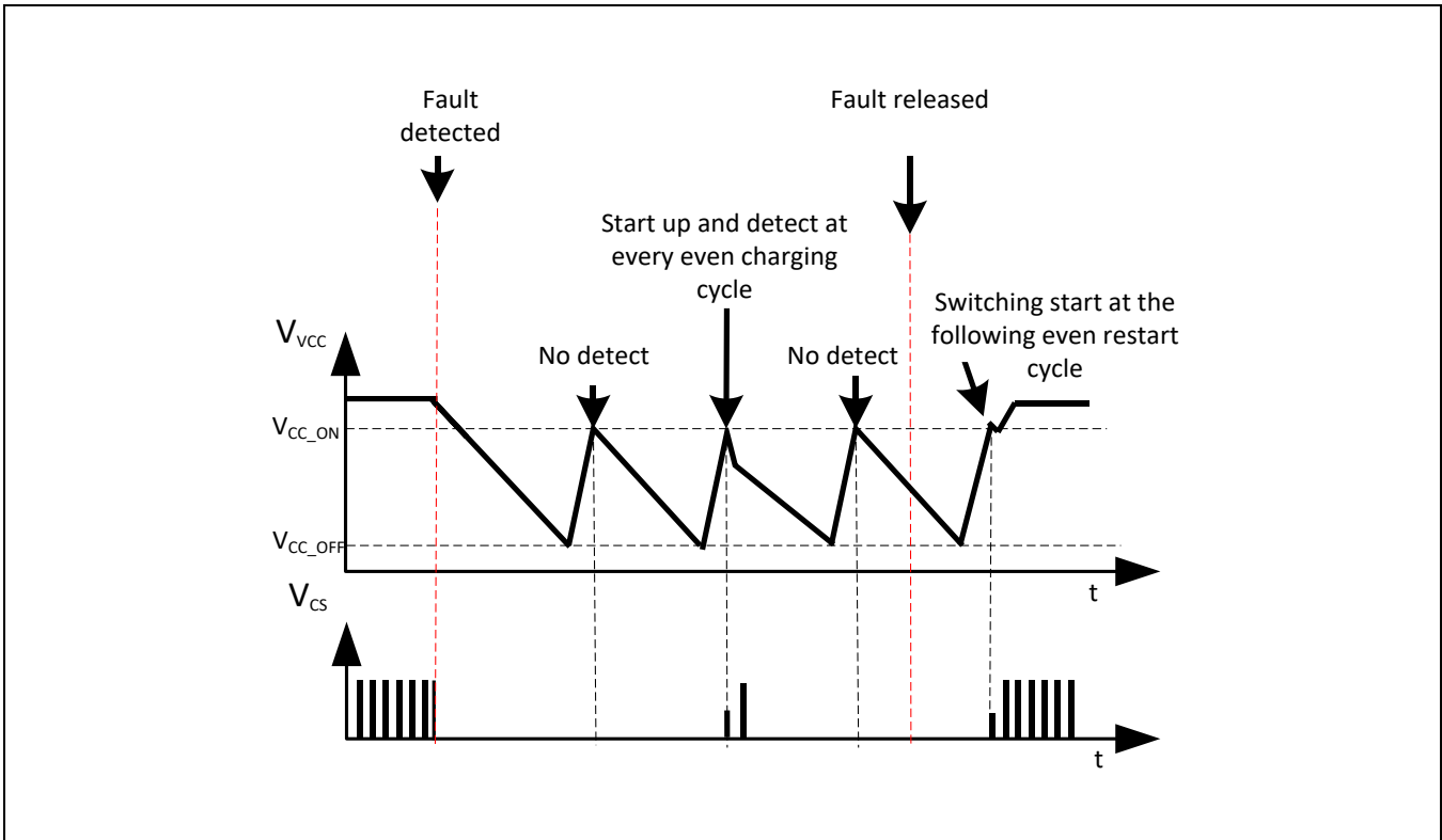
Figure 13 Odd skip Auto Restart Mode
