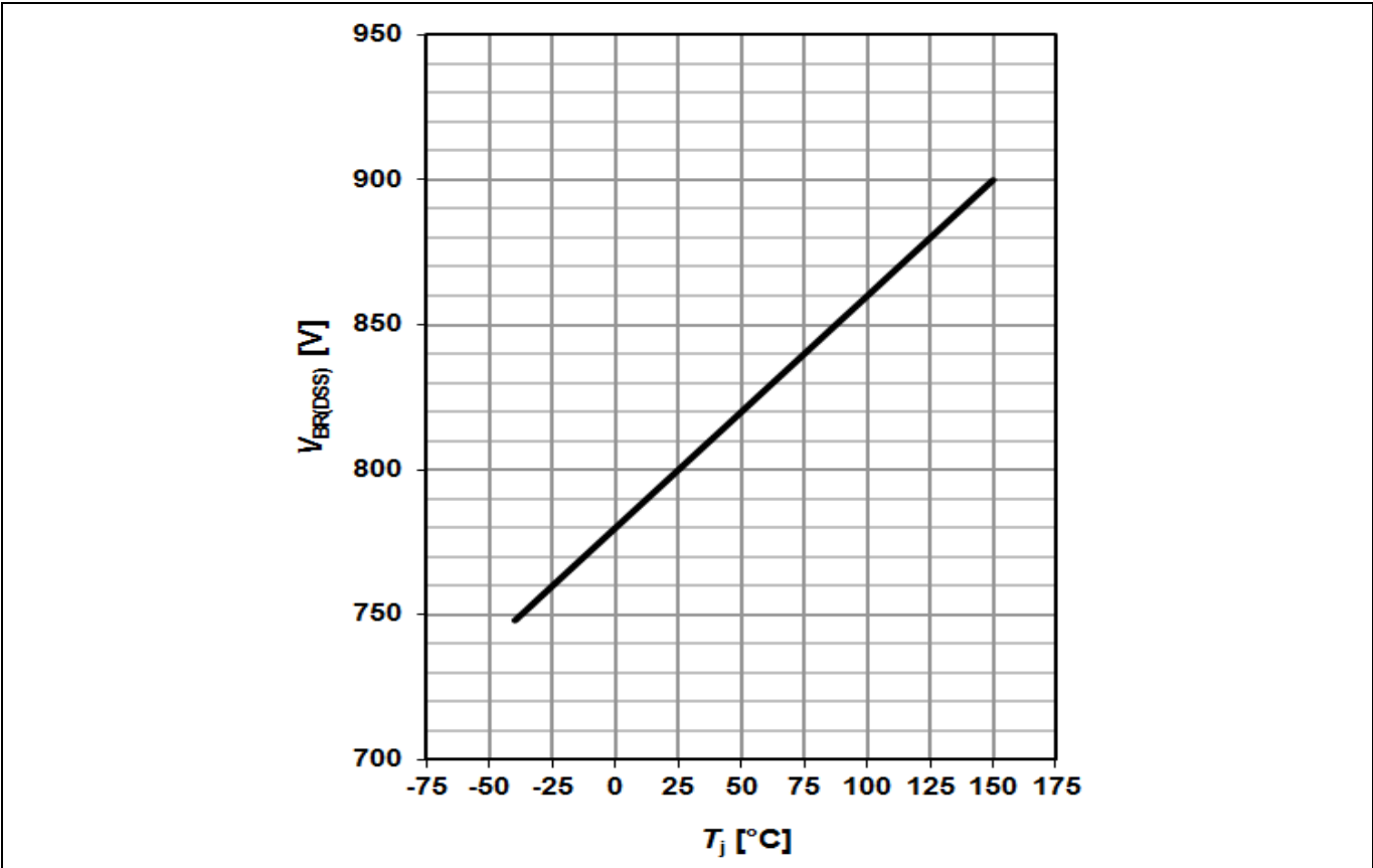
Figure 22 Drain-source breakdown voltage ICE5QRxx80BG; V_{BR(DSS)}=f(T_j) , I_D=1 mA
