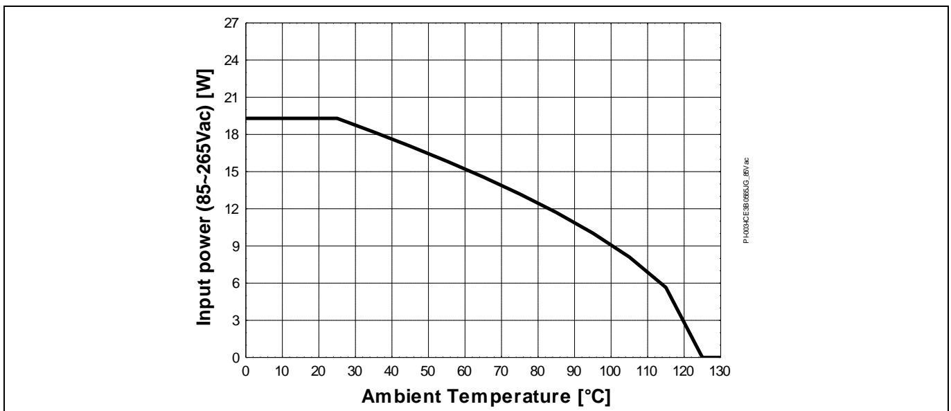
Figure 32 Input power curve V_{IN}=85 \sim 265 \text{ V}_{AC} ; P_{in}=f(T_a)
