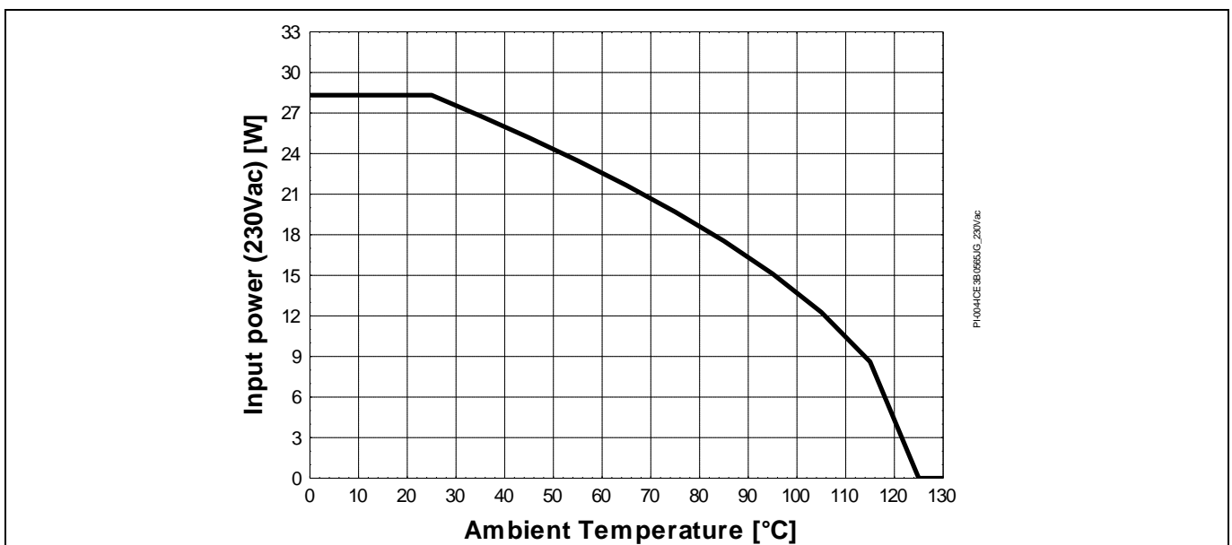
Figure 33 Input power curve V_{IN}=230 \text{ V}_{AC} ; P_{in}=f(T_a)
