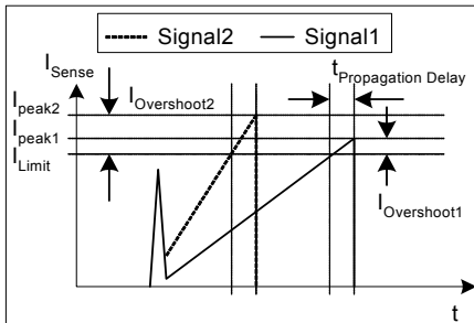
Figure 19 Current Limiting
