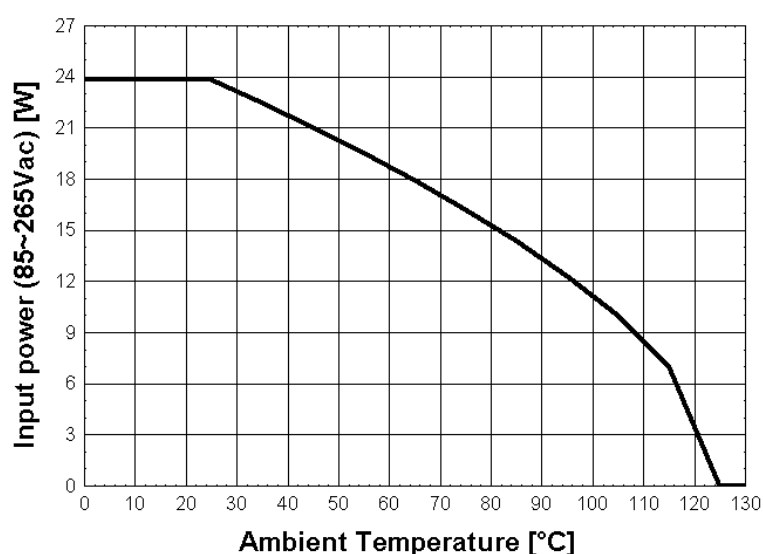
Figure 42: Input power curve V_{in}=85\sim 265V_{ac} ; P_{in}=f(T_a)
