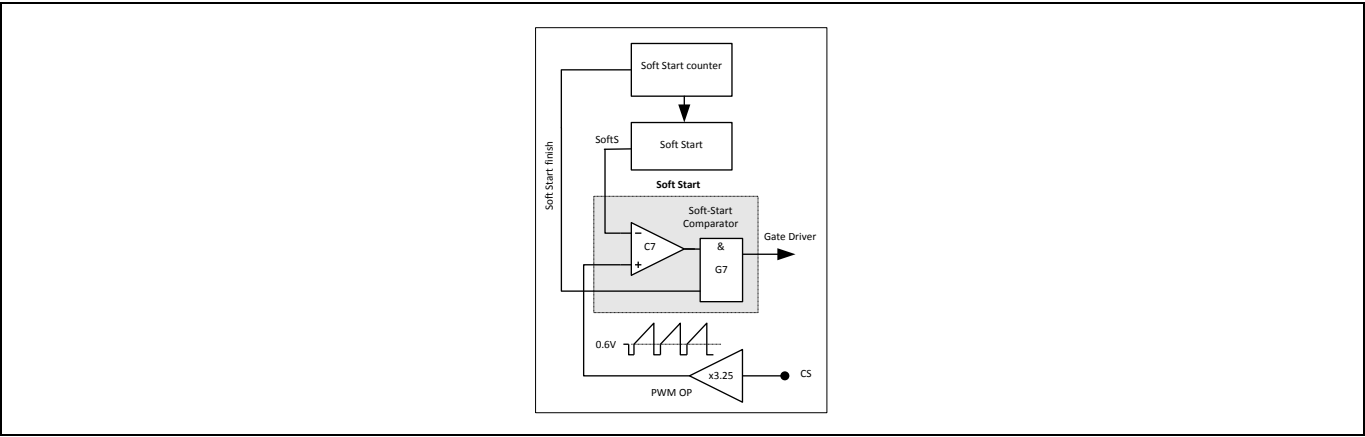
Figure 10 Soft Start
