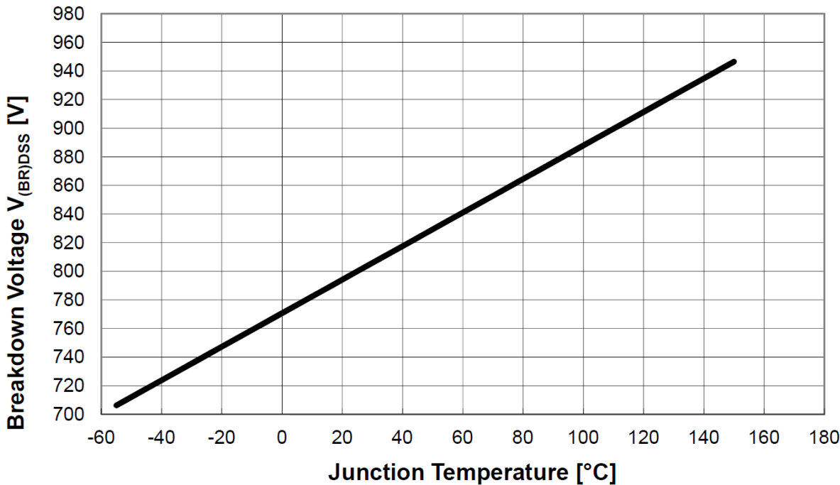
Figure 39 Drain-source breakdown voltage; V_{BR(DSS)}=f(T_j) , I_D=0.25mA
