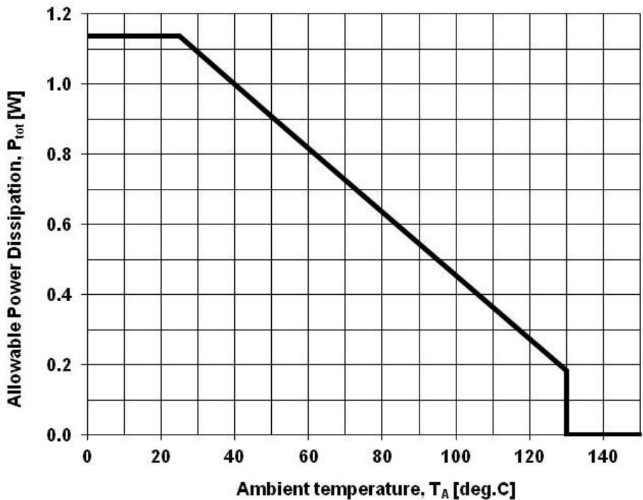
Allowable Power Dissipation for F3 CoolSET in DSO-16/12 package
