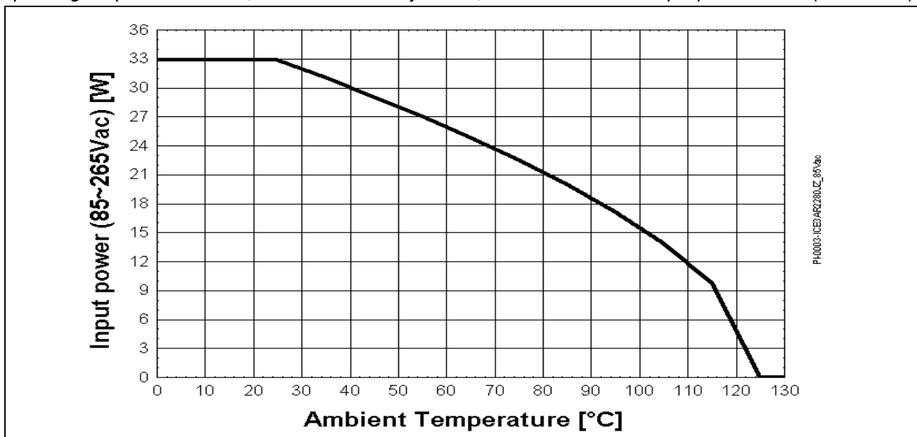
Figure 38 Input power curve V_{in}=85\sim 265\text{Vac} ; P_{in}=f(T_a)
