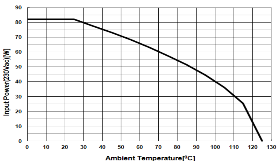
Figure 43: Input power curve V_{in}=230\text{Vac} ; P_{in}=f(T_a)
