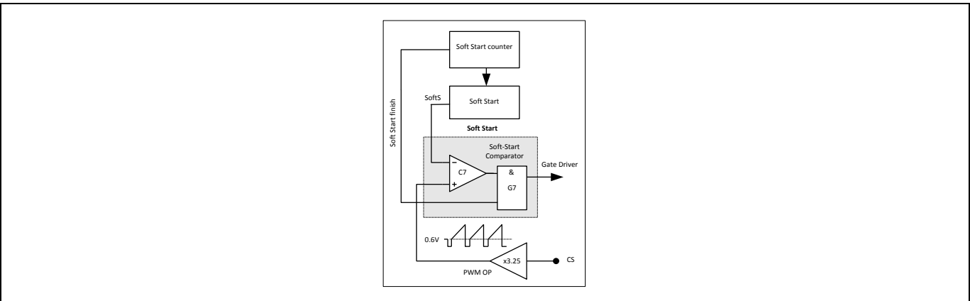
Figure 10 Soft Start
