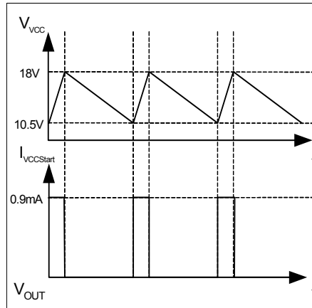
Figure 26 Signals in Latched Off Mode
