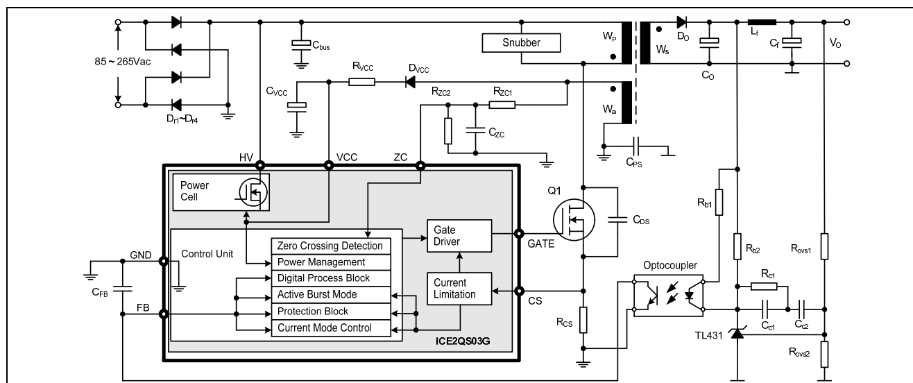
Figure 1 Typical Application
