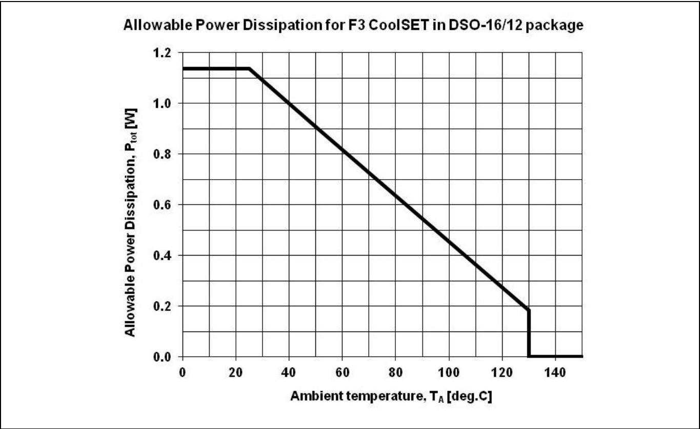
Figure 11 Power dissipation; P_{\text{tot}} = f(T_A)
