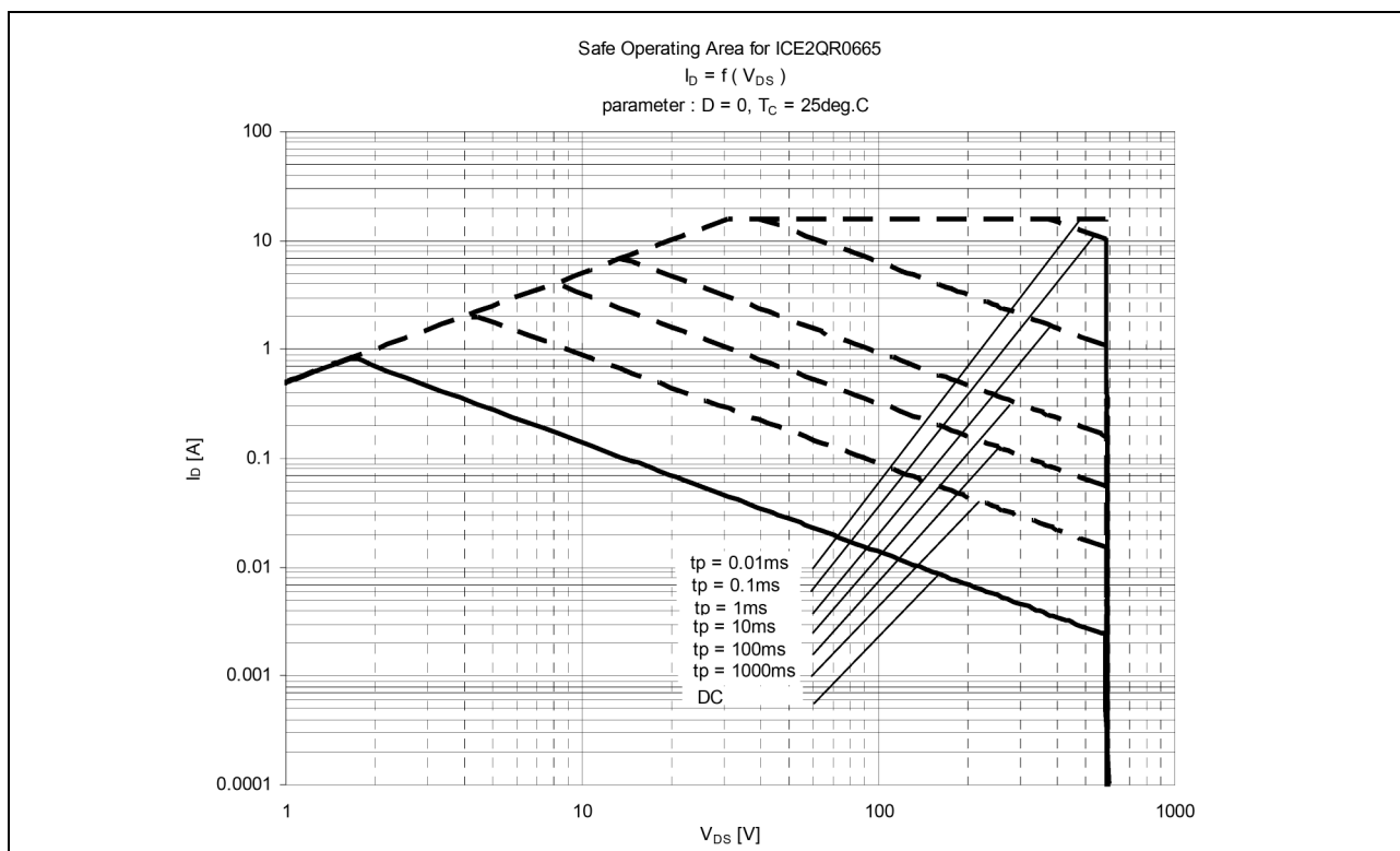
Figure 9 Safe Operating Area(SOA) curve for ICE2QR0665
