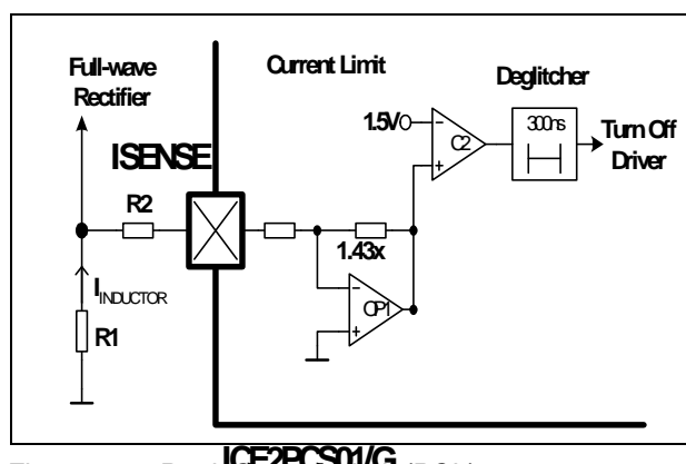
Figure 9 Peak Current Limit (PCL)
