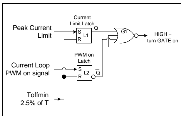
Figure 14 PWM Logic
