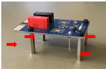
Step 5 MOSFETs placement into the socket
