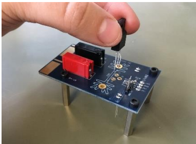
Step 5 MOSFETs placement into the socket
