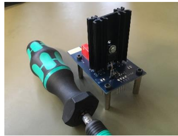
Step 5 MOSFET placement into the socket
